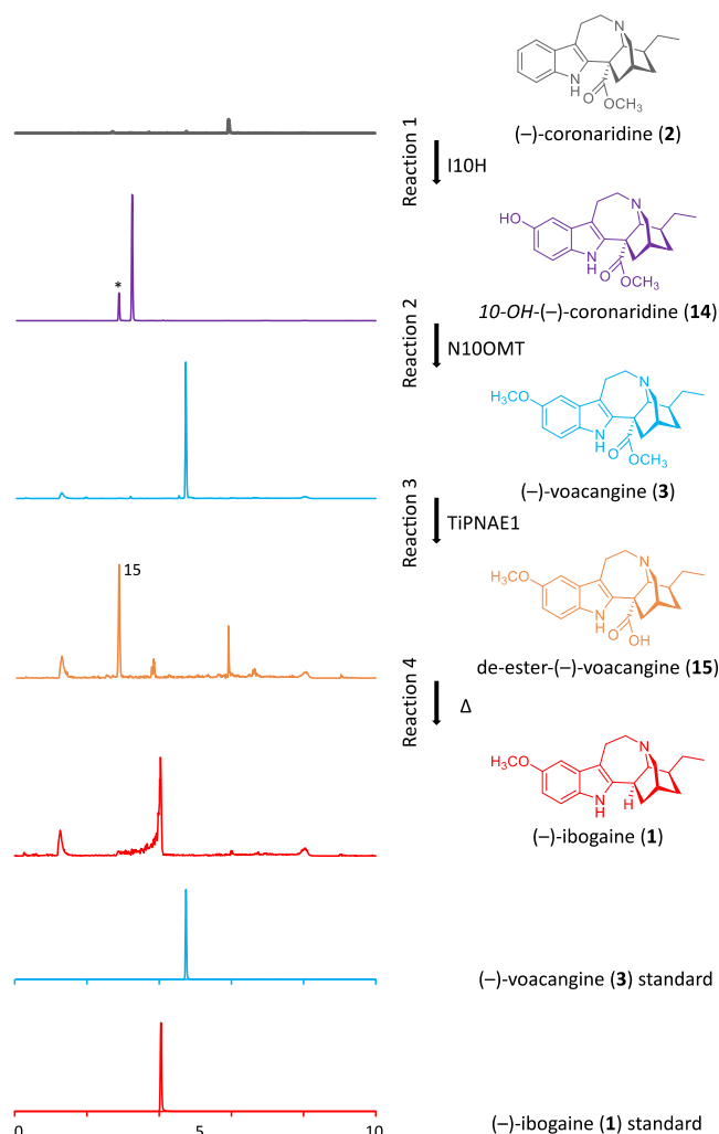
Figure 3. Formation of (–)-ibogaine (1) from enzymatically generated (–)-coronaridine (2). Peaks marked with an asterisk were products of endogenous yeast enzymes present in cultures expressing I10H.
