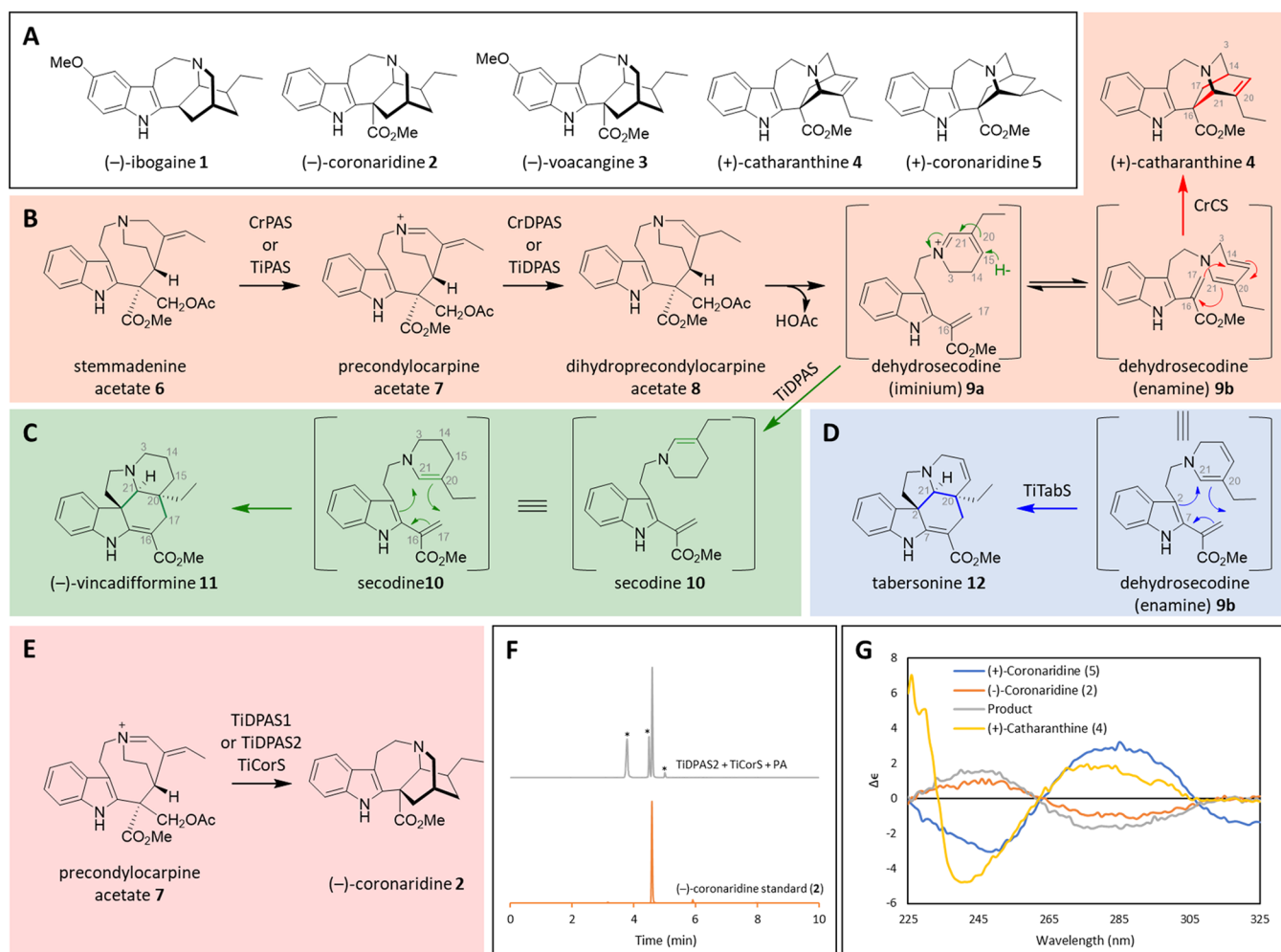
Figure 1. (+) and (-)-Iboga alkaloids. (A) Anti-addiction agents (-)-ibogaine ( 1 ) and (-)-voacangine ( 3 ) are antipodal to (+)-catharanthine ( 4 ), a precursor to the anticancer drug vincristine. (B) Biosynthesis of (+)-catharanthine ( 4 ). It is assumed that dehydrosecodine iminium 9a is initially formed, and it then tautomerizes to the enamine form 9b . (C) Biosynthesis of (-)-vincadifformine ( 11 ). (D) Biosynthesis of (-)-tabersonine ( 12 ). (E) Biosynthesis of the reduced iboga alkaloid (-)-coronaridine ( 2 ) directly from precondylocarpine acetate ( 7 ). (F) LC-MS chromatogram showing formation of (-)-coronaridine ( 2 ) after incubation of precondylocarpine acetate ( 7 ) (50 \mu M) with TiDPAS2 (1 \mu M), TiCorS (5 \mu M), and NADPH (8 equiv). Peaks marked with an asterisk are uncharacterized side products ( m/z 339) that decomposed during isolation attempts. (G) CD spectra of enzymatically produced coronaridine compared to authentic standards.
