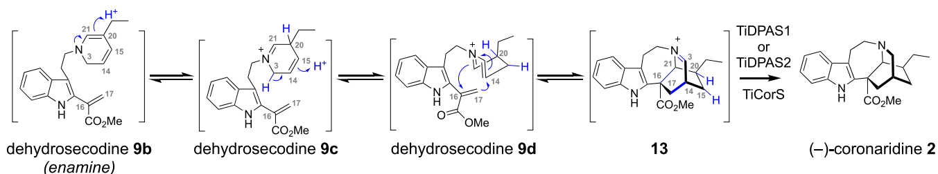
Figure 2. Biosynthesis of (-)-conaridine ( 2 ) by TiDPAS1/2 and TiCorS. One plausible chemical mechanism for formation of the (-)-conaridine ( 2 ) scaffold that is consistent with experimental evidence.
